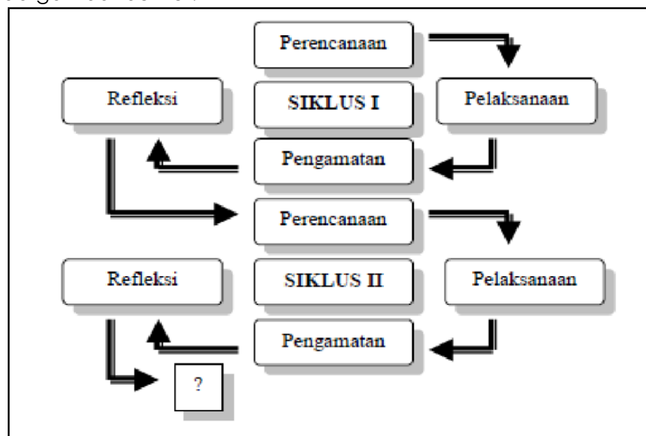
Gambar 1. Prosedur Penelitian
