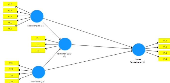
Figure 1. PLS-SEM Model Specifications
