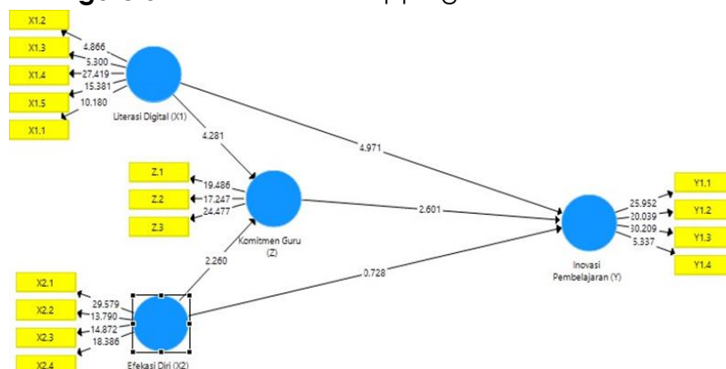
Figure 3. PLS-SEM Bootstrapping Estimation Results
