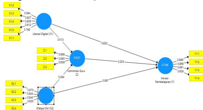
Figure 2. PLS-SEM Algorithm Estimation Results
